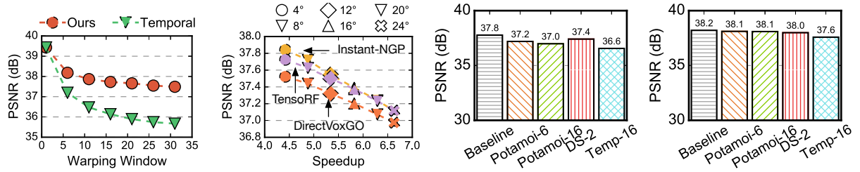
Fig. 19. The accuracy sensitivity to window size between POTAMOI and the warping-based method.
