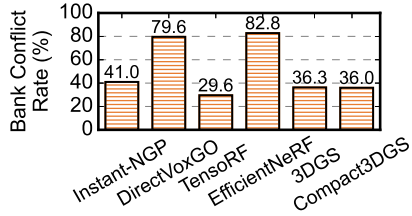
Fig. 6. SRAM bank conflict rate in Feature Gathering ( G ), assuming 16 banks and 16 concurrent ray queries.
