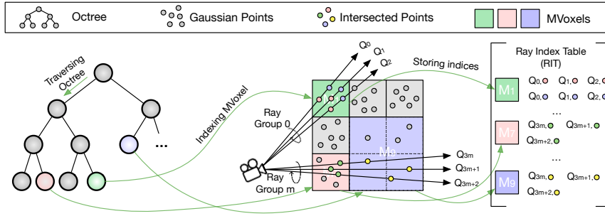
Fig. 13. Modified Indexing ( \mathcal{I} ) stage for unstructured representations [12, 33, 74]. We merge adjacent low-density MVoxels for better on-chip buffer utilization. An offline-built octree is used to help MVoxel traversal.
