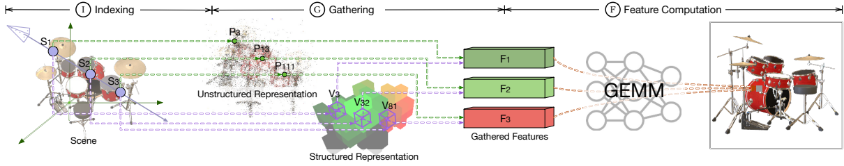
Fig. 1. The rendering pipeline of today’s NeRFs consists of three stages: Indexing ( \mathcal{I} ), Feature Gathering ( \mathcal{G} ), and Feature Computation ( \mathcal{F} ). For NeRFs with structured representations, each ray first samples points ( S_1, S_2 , and S_3 ) along the ray direction. Each ray sample gathers and interpolates 3D features from eight vertices of the intersected voxel ( V_3 , and V_{32} , and V_{81} ) to obtain features ( F_1, F_2 , and F_3 ), as highlighted in purple. For NeRFs with unstructured representations, each ray directly intersects with Gaussian points ( P_3, P_{13} , and P_{111} ) to obtain features, as highlighted in green. Then, the features are fed into the GEMM-based computation to get the partial pixel values, as highlighted in orange. The final pixel value is summed from all partial pixel values [48].
