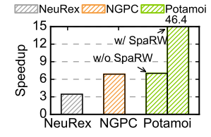
Fig. 27. Performance comparison against prior works.
