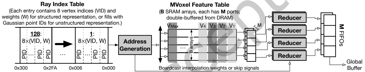
Fig. 17. Gathering unit. Each RIT entry stores the information of a ray sample. For structured representations, each entry has eight vertex IDs (VIDs) as well as the corresponding weights ( W ) for trilinear interpolation. For unstructured representations, each entry contains a single ID of the intersected Gaussian point (PID). The Address Generation logic uses the VID/PIDs to access the corresponding features from the MFT, which stores the features of a MVoxel using the channel-major layout. The VFT has B individual SRAM arrays, each has M ports, supporting retrieving features for M ray samples simultaneously. Trilinear interpolation is supported by B \times M number of reducers to calculate the final features for M ray samples. The weights are broadcast to the reducers. A FIFO holds the feature results before writing to the Global Feature Buffer in Fig. 16.
