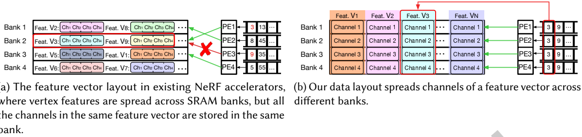
Fig. 15. A comparison between the original feature vector layout (Fig. 15a) and our data layout (Fig. 15b). The example has four banks and four concurrent PEs. In Fig. 15a, a bank conflict occurs when PE 1 and PE 3 (each collecting features for a different ray sample) access two different features from bank 2. Our data layout (Fig. 15b) eliminates bank conflicts by 1) spreading channels across banks and 2) having each PE collect a particular channel across different ray samples.
